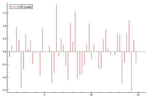
Figure 4: Model residuals.
