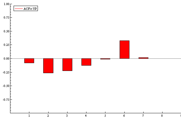
Figure 1: Autocorrelation function.
