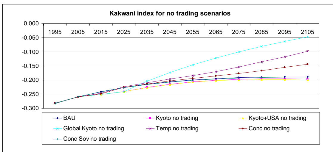
Figure 4 Kakwani index.
