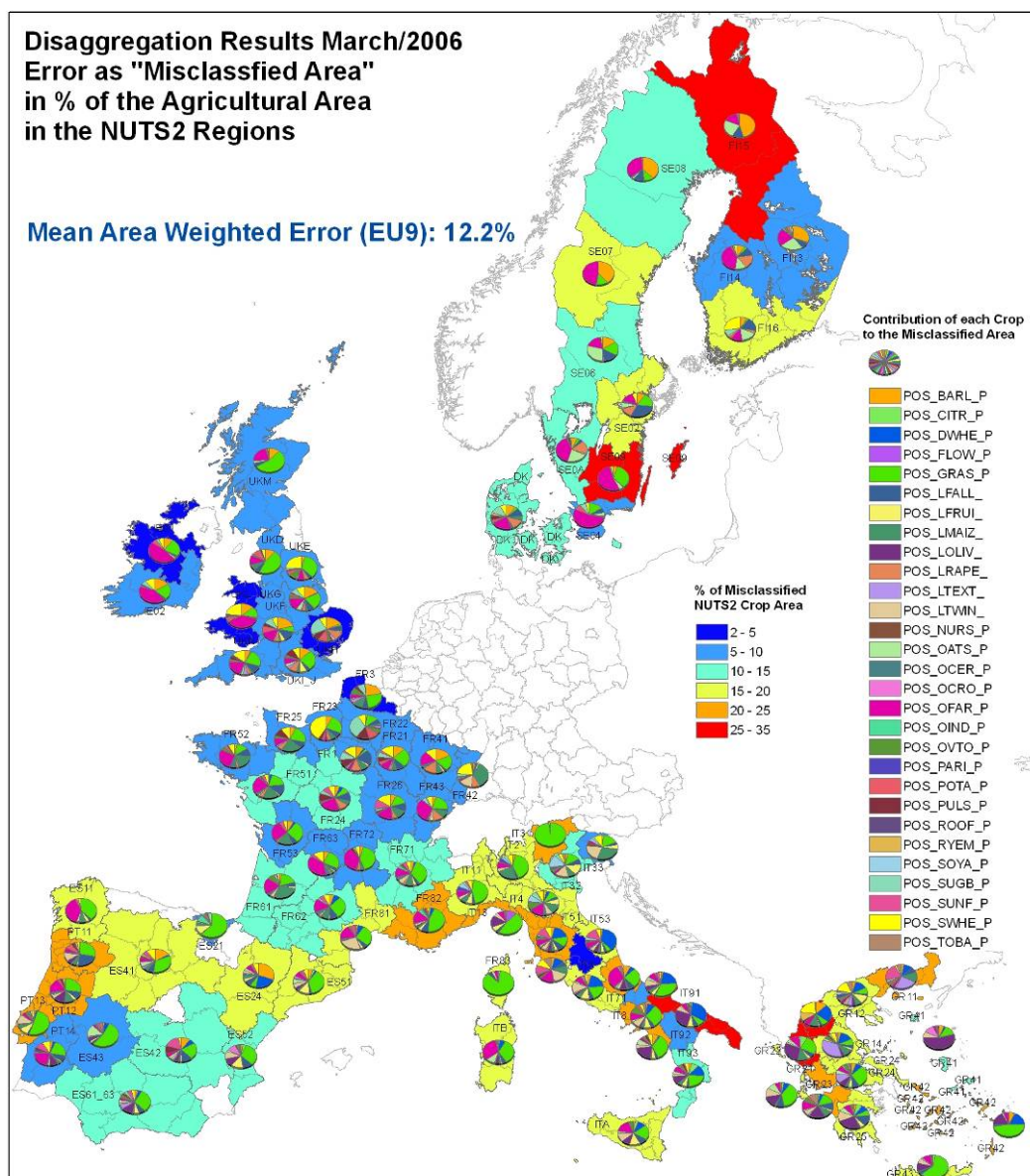
Figure 2.3 Comparison of disaggregation results with the statistical information at Nuts 2 level.
