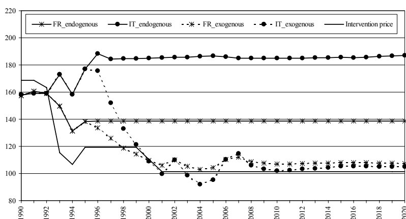
Figure 4. French and Italian price projections according to the two price formation specifications: baseline
