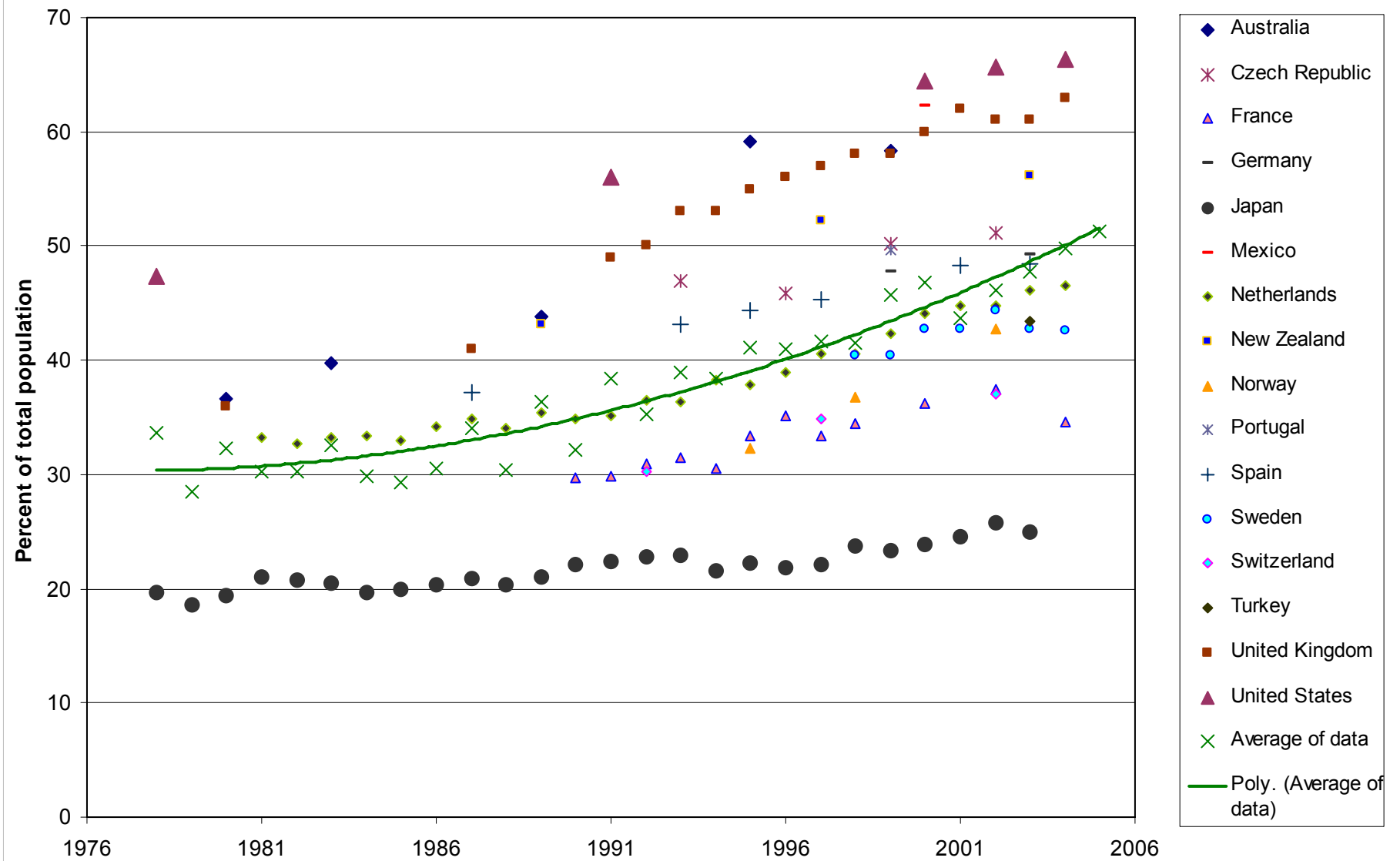
Figure 6. Overweight and obese populations in some OECD countries
