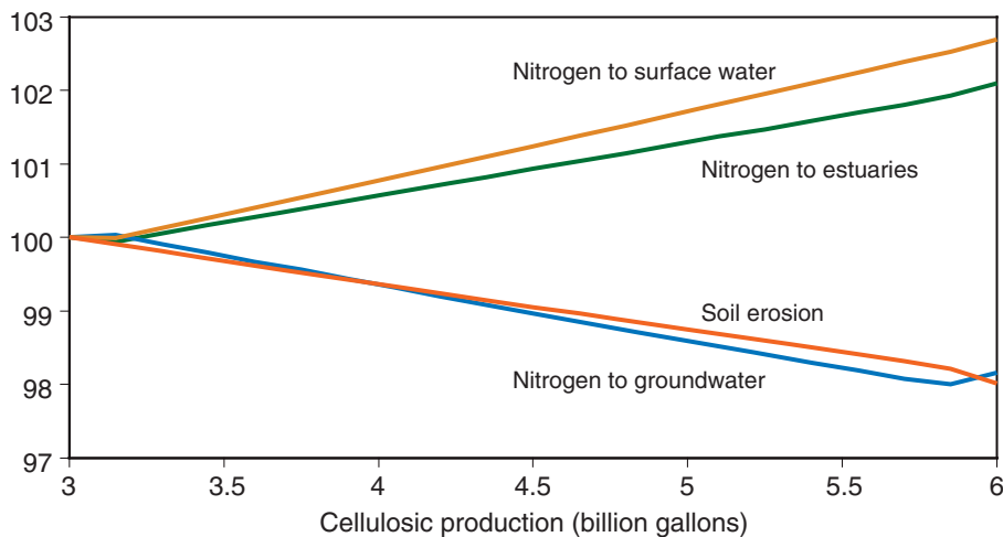
Figure 16 Changes in environmental indicators relative to 3 billion gallons of cellulosic ethanol production
