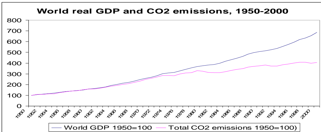
Fig 9 – CO 2 and GDP trends
