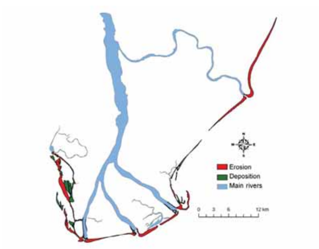
FIGURE 13. A contour of the Krishna Delta showing areas of erosion and deposition during the period between 1977 and 2000.
