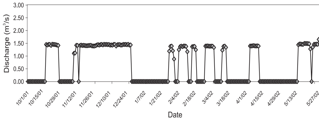
FIGURE A11. Daily flow measurement at Lalian middle outlet, LJCS-Pakistan.
