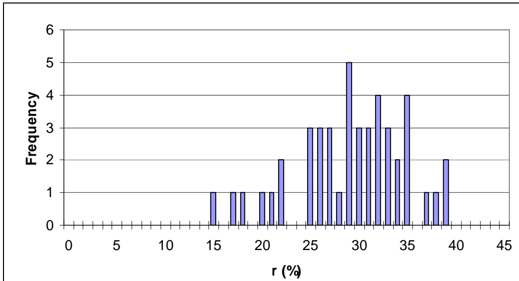
Figure 1. Histogram of the own state IRR's, (\hat{r}) – Model 1
