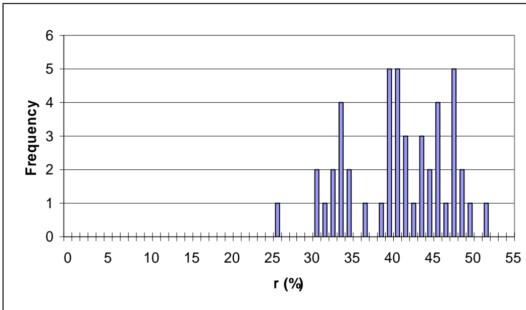
Figure 2. Histogram of the social IRR's, (\hat{r}_1) – Model 1
