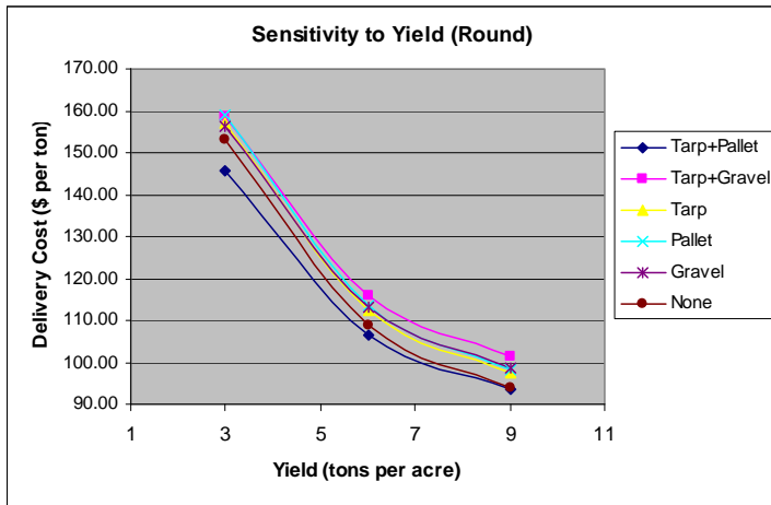
Figure 2. Sensitivity of delivered costs at 200-day of storage to switchgrass yield
