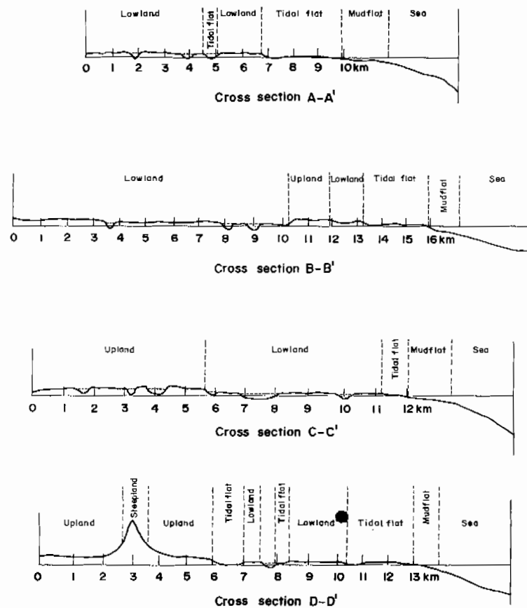
Fig. 1.4. Cross-sectional profiles of the coasts along Ban Don Bay.
