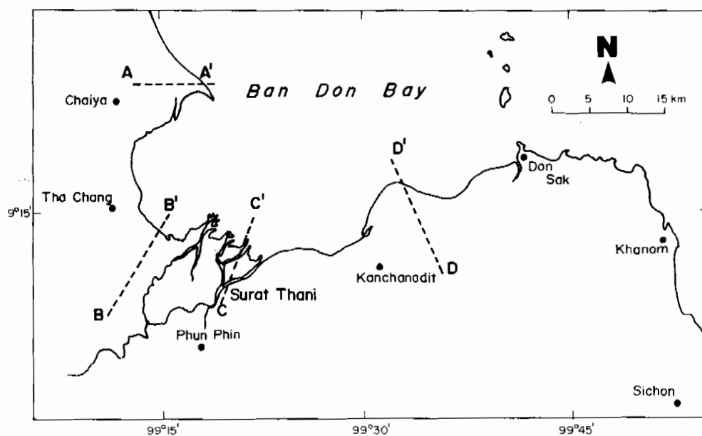
Fig. 1.3. Study site in Ban Don Bay with the cross-sectional areas marked.
