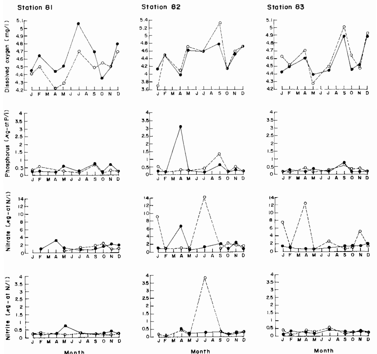
Fig. 2.5. Monthly distribution of (top to bottom): dissolved oxygen, phosphorous, nitrate and nitrite at stations 81, 82 and 83 in 1985.
