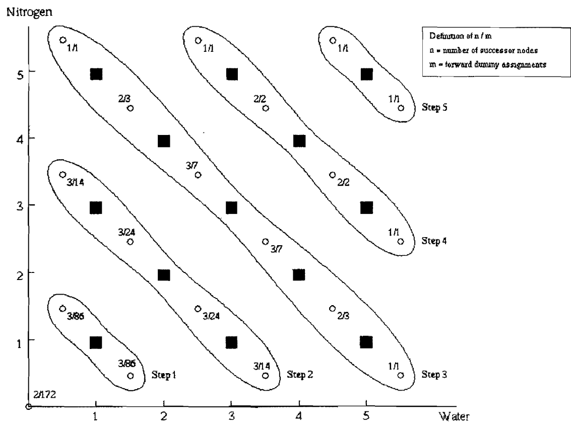
Figure 2. Bounding the number of dummy configurations by backwards induction
