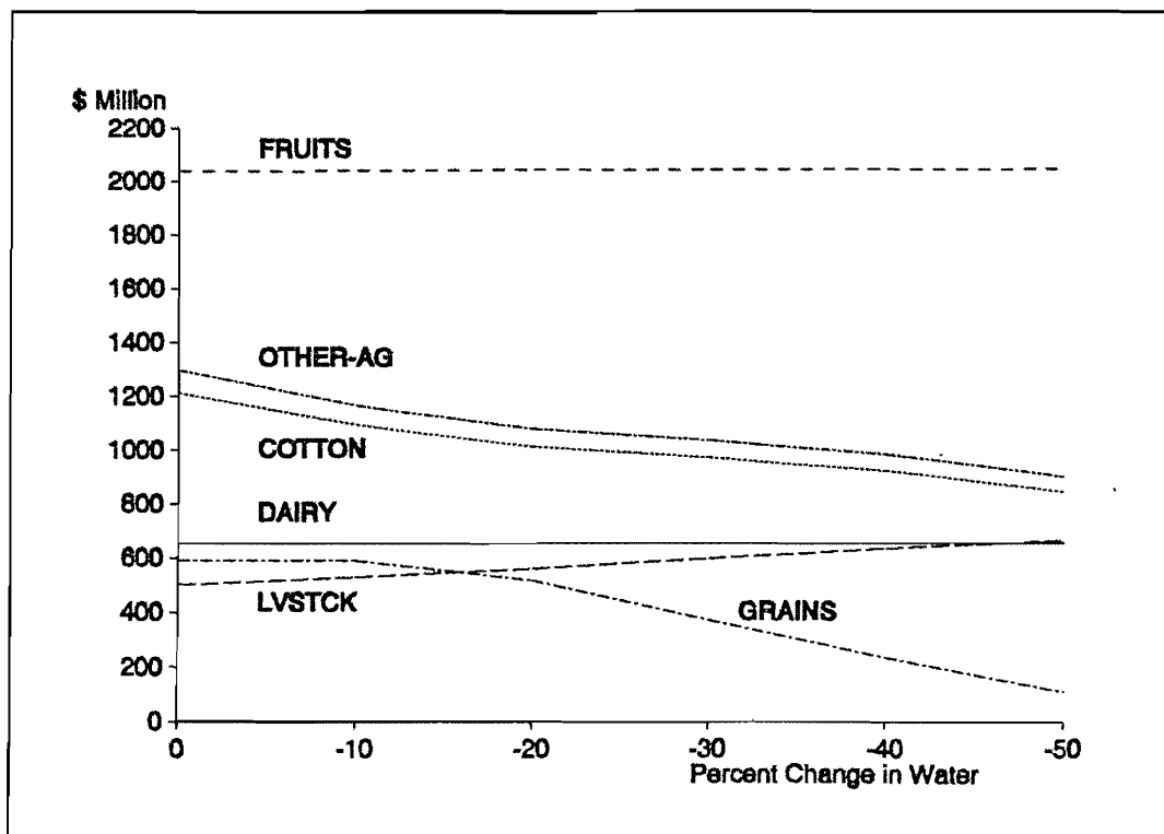
Figure 5: Output, High Substitution Elasticities
