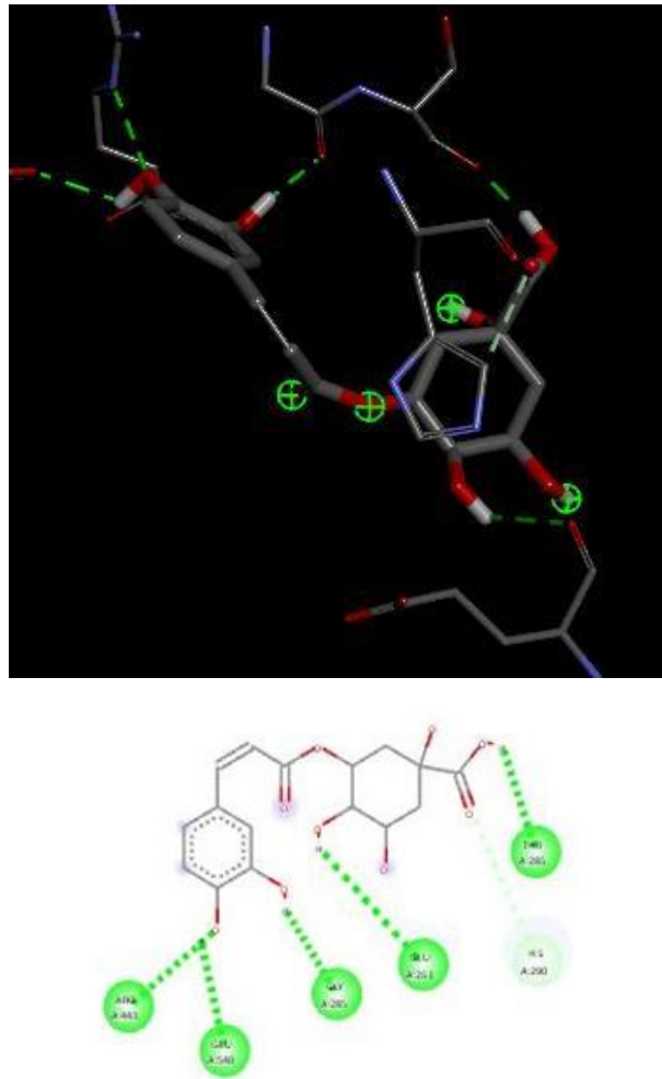
Figure 3.7: 2D receptor-ligand interaction of Chlorogenic acid ( Colocasia esculenta ) in the binding site of the receptor of \alpha -amylase (PDB ID: 4GQQ).
