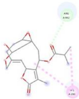
Figure 3.13: 2D receptor-ligand interaction of vernomygdin ( Vernonia amygdalina ) in the receptor's binding site of \alpha -amylase (PDB ID: 4GQQ)
