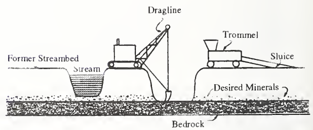
Figure 2-5: Placer Mining
