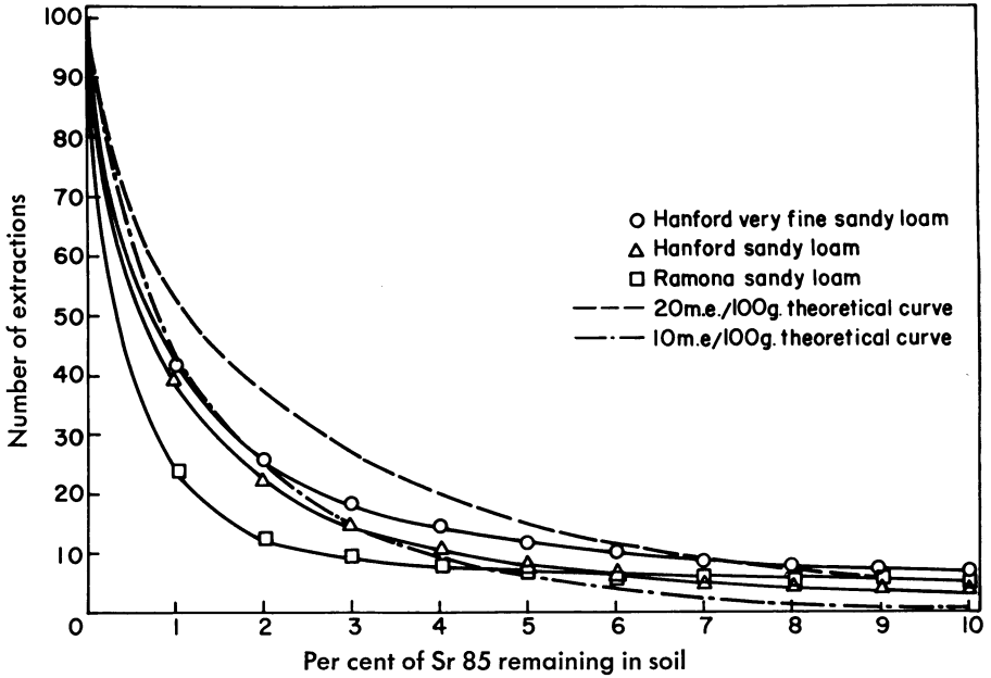
Fig. 2. Extraction of Sr 85 from Hanford and Ramona soils with 1N NH 4 Ac
