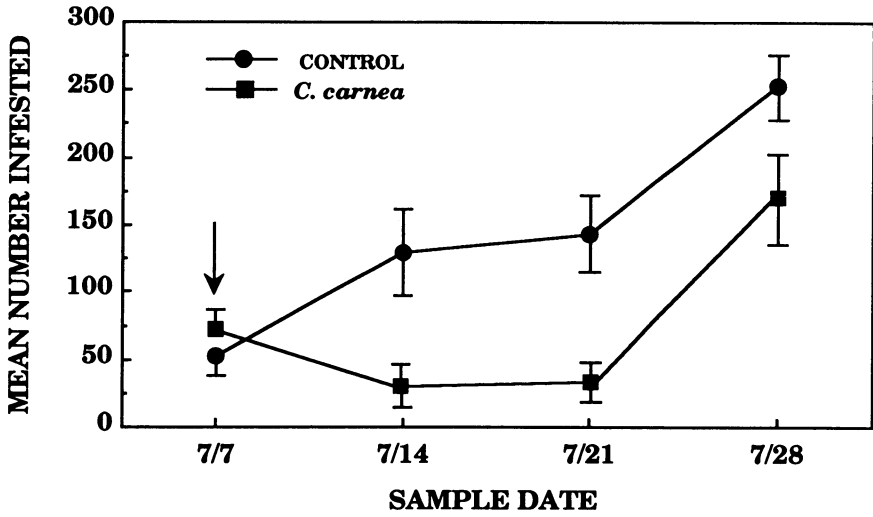
Fig. 39. Mean (SEM) number of seedlings infested by M. kinseyi in control and lacewing release plots. Arrow indicates date of the release of prefed larvae of C. carnea . Results for paired "t" test with d.f. = 18: 7/7, t = 1.31 , P = 0.21 ; 7/14, t = 5.51 , P = 0.0001 ; 7/21, t = 5.28 , P = 0.0001 ; 7/28, t = 2.94 , P = 0.009 .
