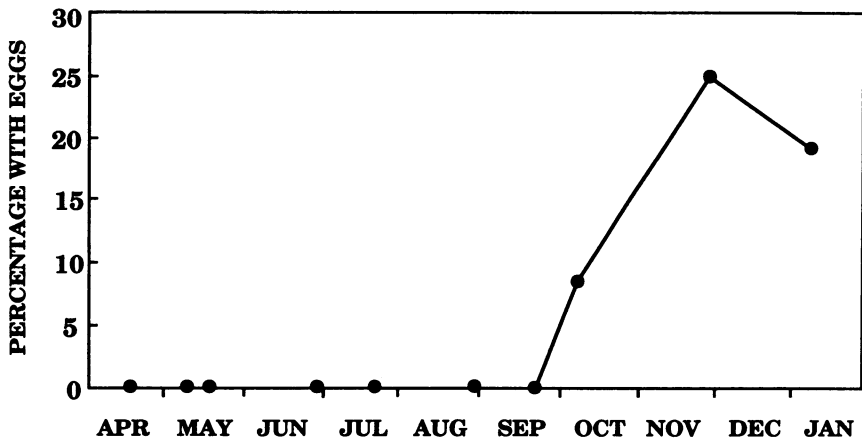
Fig. 11. Percentage of second-year seedlings with one or more eggs of M. kinseyi during 1989-90.
