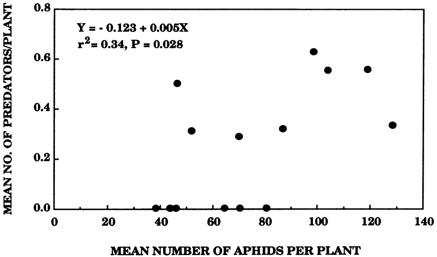
Fig. 17. Relationship between mean number of predators (eggs + larvae) and mean number of M. kinseyi per infested, first-year seedling in the ecology plot during 1989.
