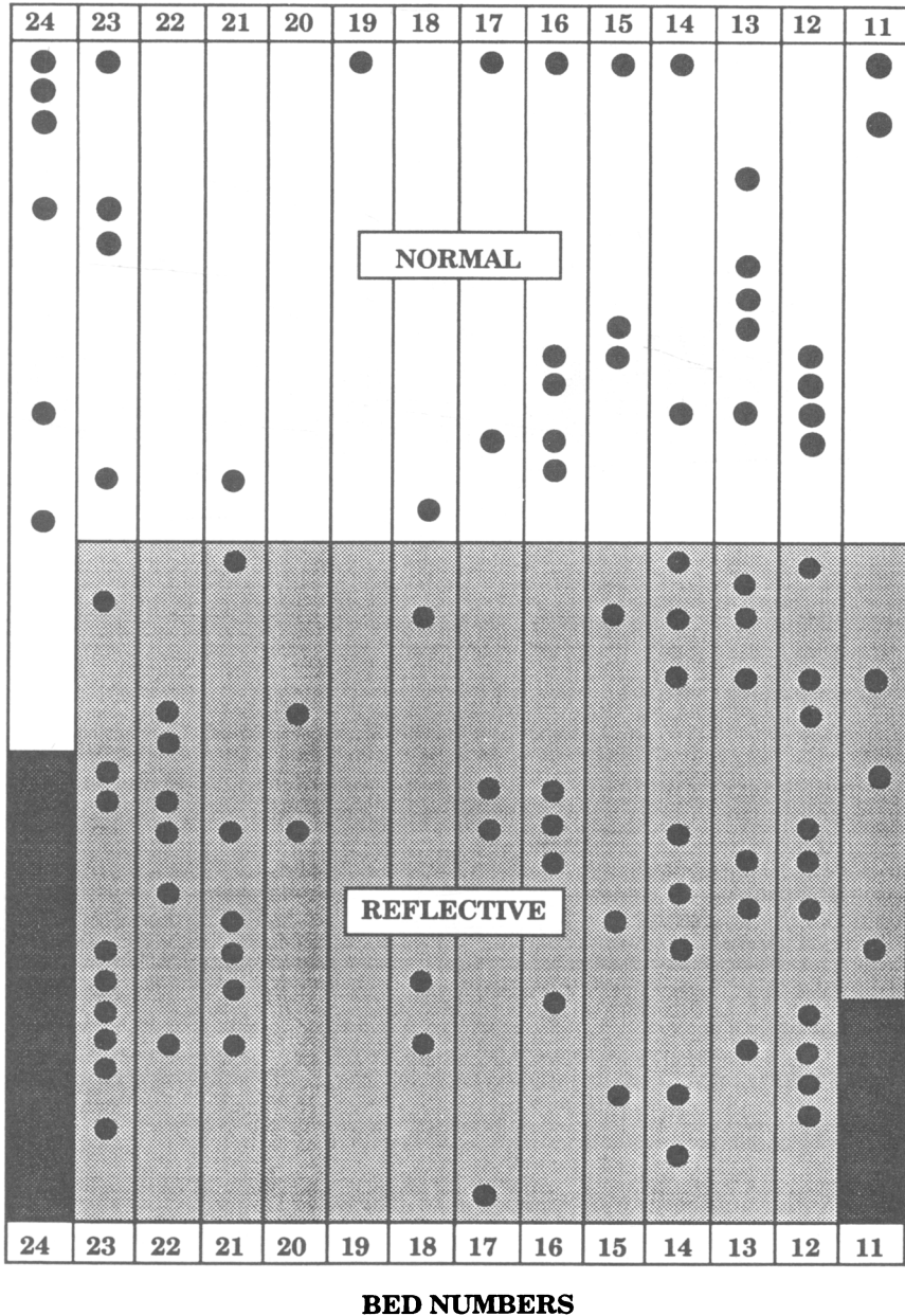
Fig. 36. Approximate spatial distribution of infested patches of first-year seedlings in the white-fir planting during 1992 in relation to normal vs. reflective lath shading. Heavily shaded portions of the latter were not planted to white fir.
