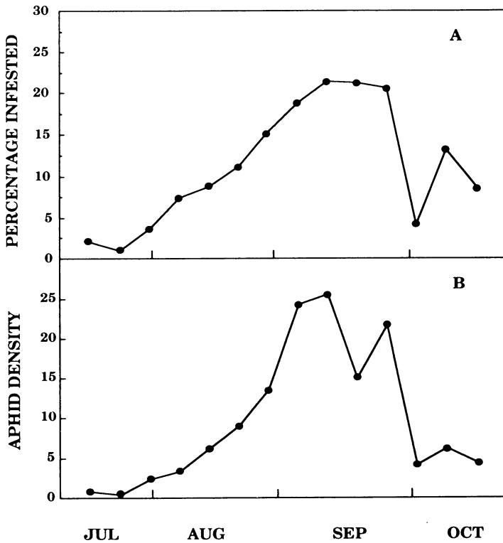
Fig. 15. Overall percentage of infested, first-year seedlings (A) and mean density ( M. kinseyi per plant) (B) in the ecology plot during 1989.
