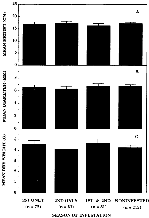
Fig. 20. Relationship between mean (SEM) height, stem diameter, and dry weight of marked seedlings at harvest, and the season in which the indicated seedlings were infested by M. kinseyi . Results for one-way analysis of variance with df = 3, 384 : (A) F = 0.25, P = 0.86 ; (B) F = 0.32, P = 0.81 ; (C) F = 0.54, P = 0.65 .
