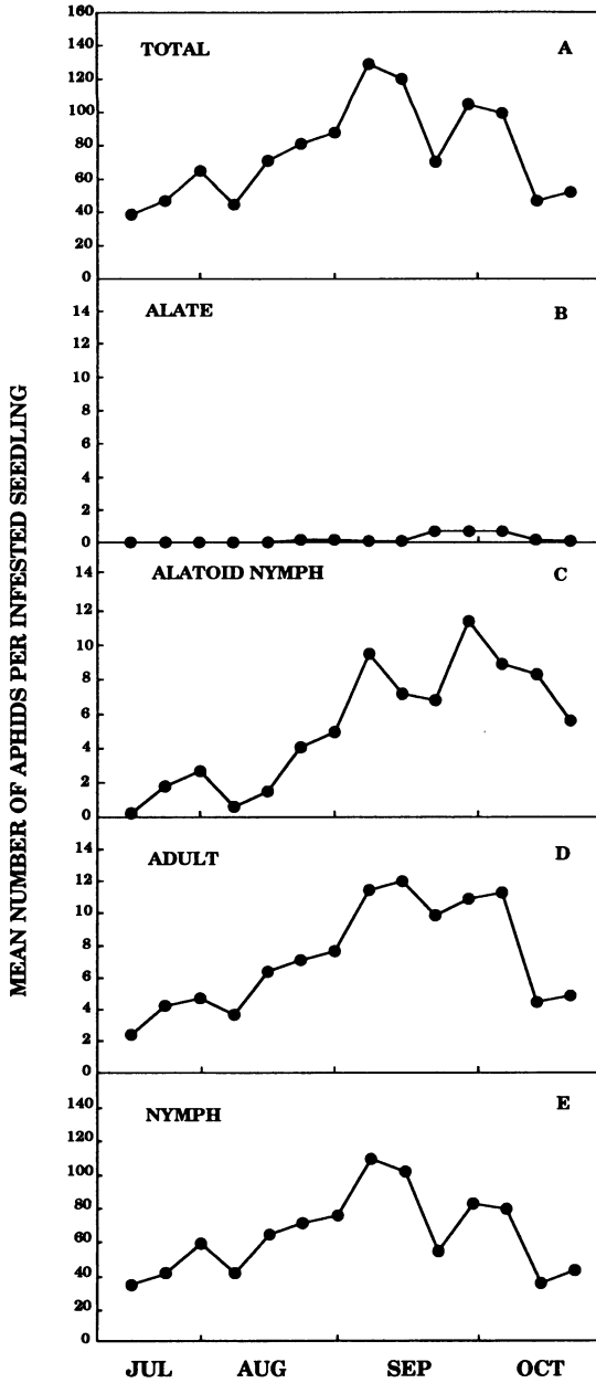
Fig. 13. Mean number of M. hinsey per infested, first-year seedling in the ecology plot during 1989.
