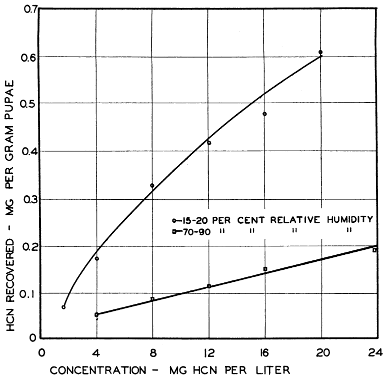
Fig. 6.—Effect of relative humidity on the recovery of HCN from walnut-husk-fly pupae. The time of exposure was 40 minutes, and the temperature 75° F.
