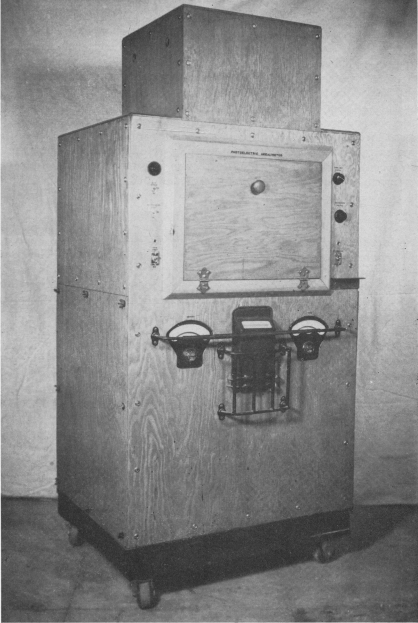
Fig. 3.—Photoelectric arealimeter.
