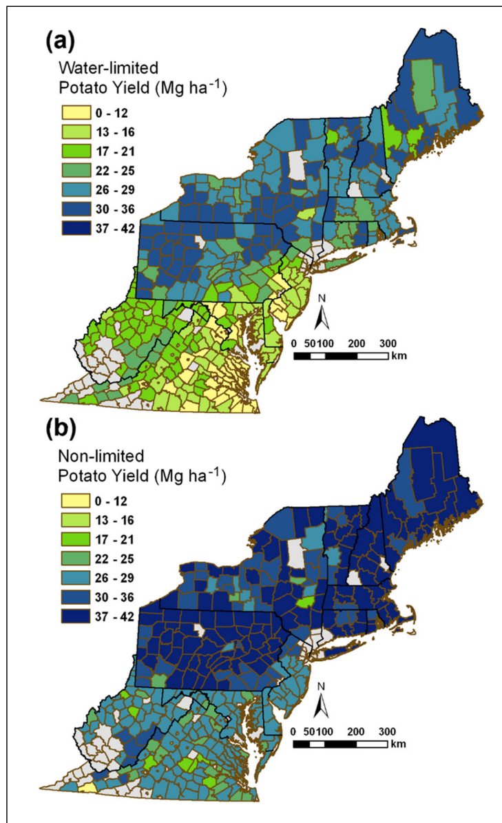
Figure 9. Simulated Potato Yield under (a) Water-Limited and (b) Non-Limited Conditions in the Eastern U.S. under Historical Climatic Conditions Results were spatially aggregated from 16 to 30m resolution
