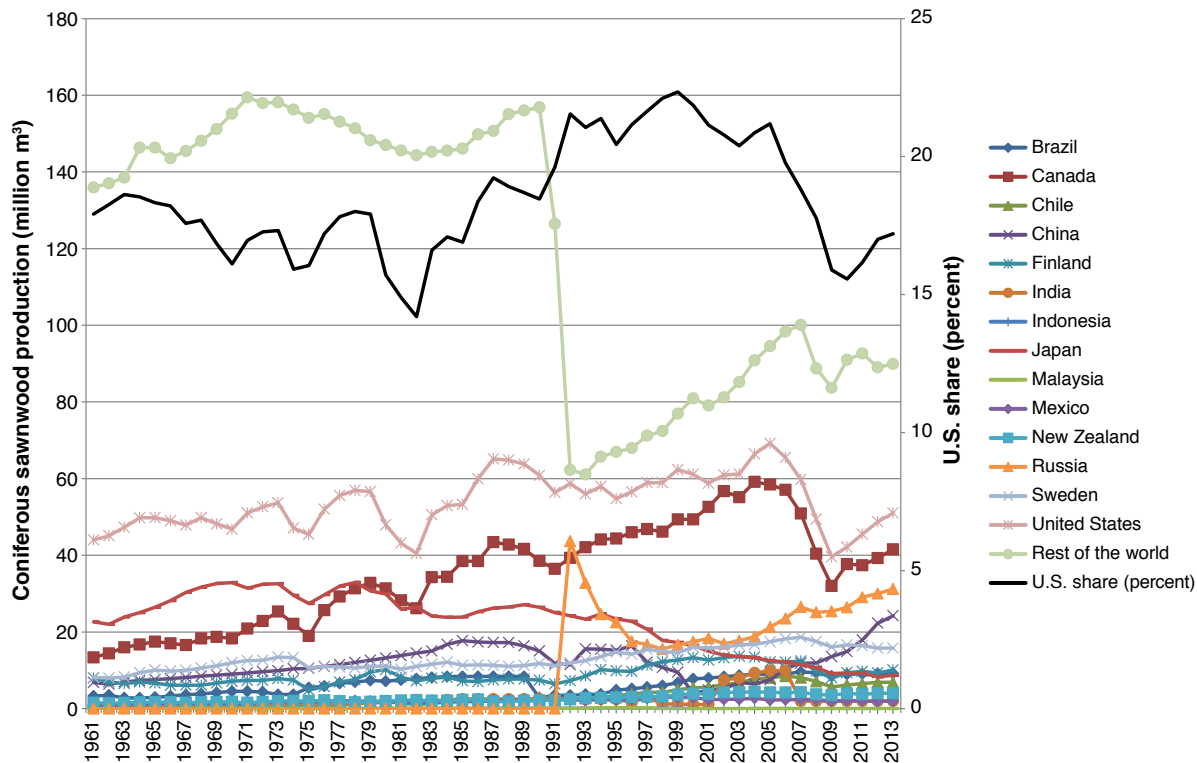
Figure 21—Coniferous sawnwood production by country and rest of the world with U.S. share of global output, 1961–2013 (Source: Food and Agricultural Organization of the United Nations 2014a). The discontinuity in the rest of the world output reflects the separate reporting of the Russian Federation States and remaining former Soviet States beginning in 1992.
