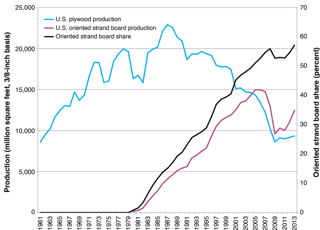
Figure 8—Production of plywood and oriented strand board in the United States, 1961-2013 (Sources: Adair 2010, APA 2014).
