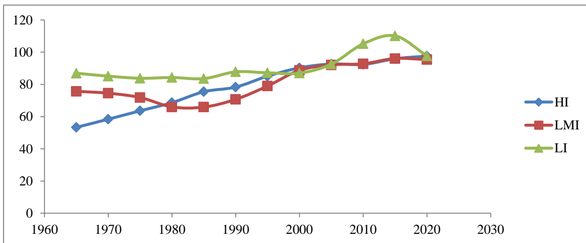
Fig. 1 Trend of Agricultural Total Factor Productivity (A-TFP) from 1960 to 2020 in high income, lower middle income and low-income countries
