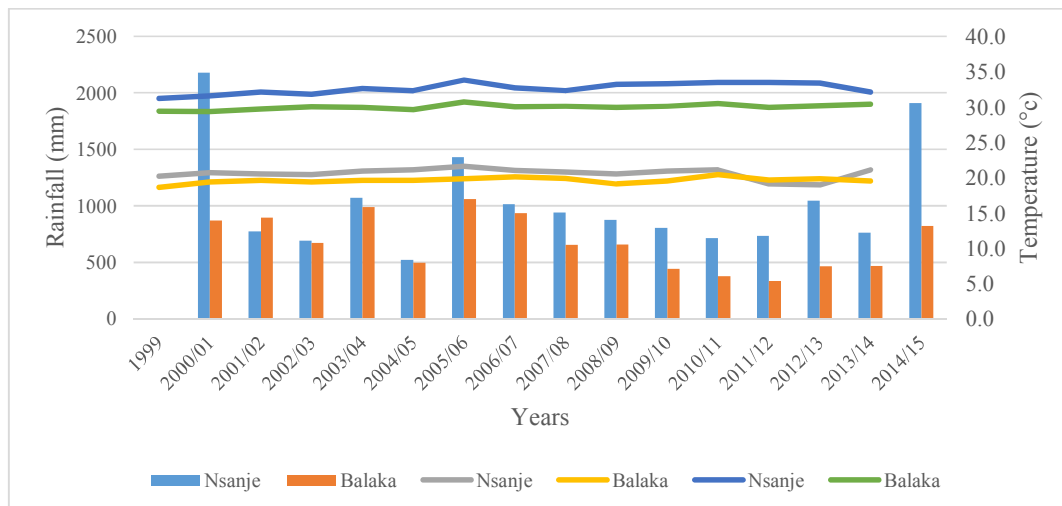
Fig. 2. Minimum and maximum temperatures and rainfall for Nsanje (Long –35.27; Lat - -16.95; 60m above sea level) and Balaka (Long – 34.97; Lat - -14.98; 625 m above sea level)
