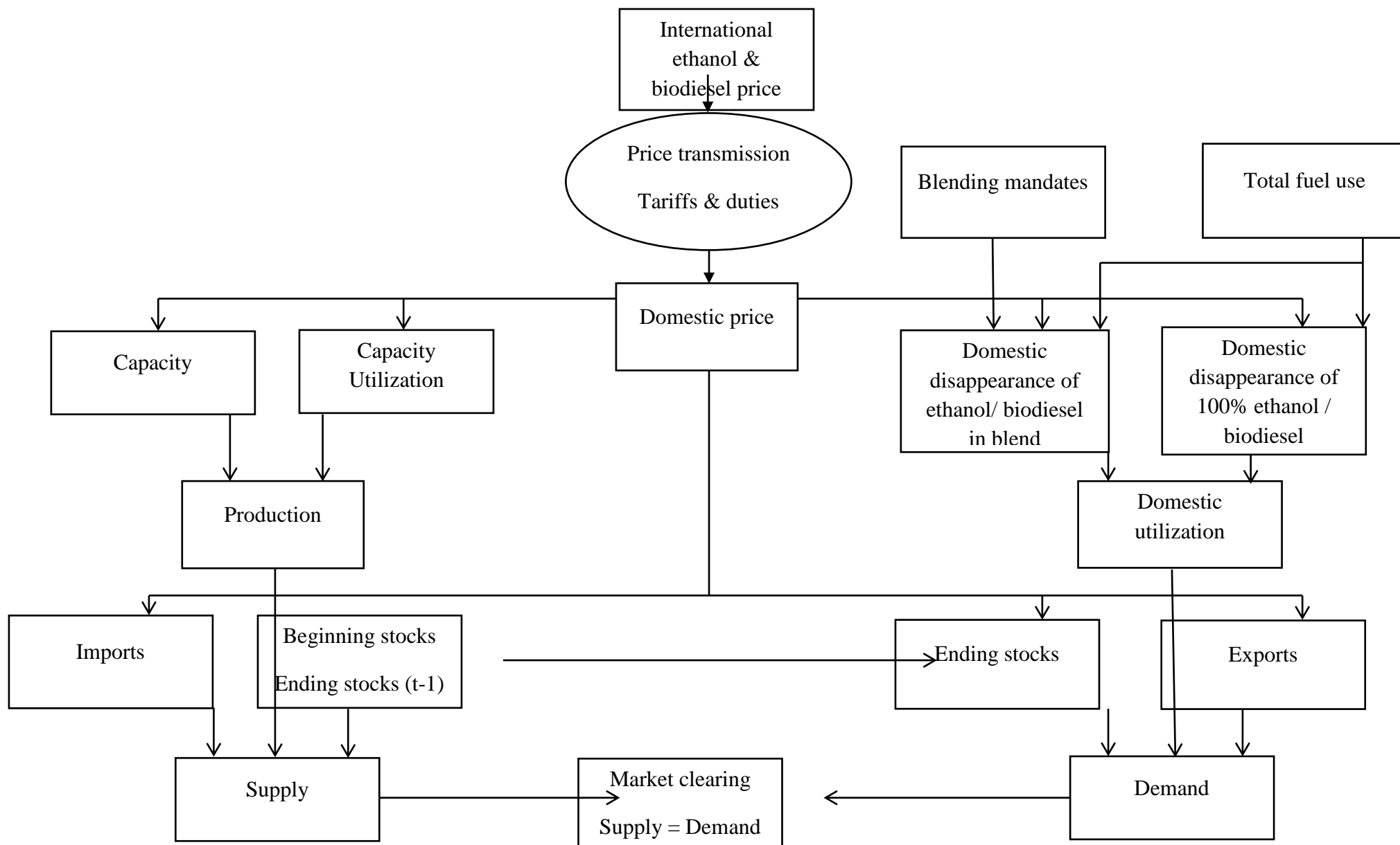
Figure 12. Schematic representation of an individual market within the international biofuels model
