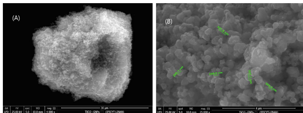
Figure 6. SEM micrograph of TiO 2 /GnPs 1% at 4000X magnification in A and 25000X in B.
