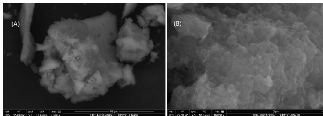
Figure 7: SEM micrograph of TiO 2 -Al 2 O 3 /GnPs 1% at 2500X magnification in A and 40 000X in B.
