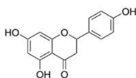
Apigenin
