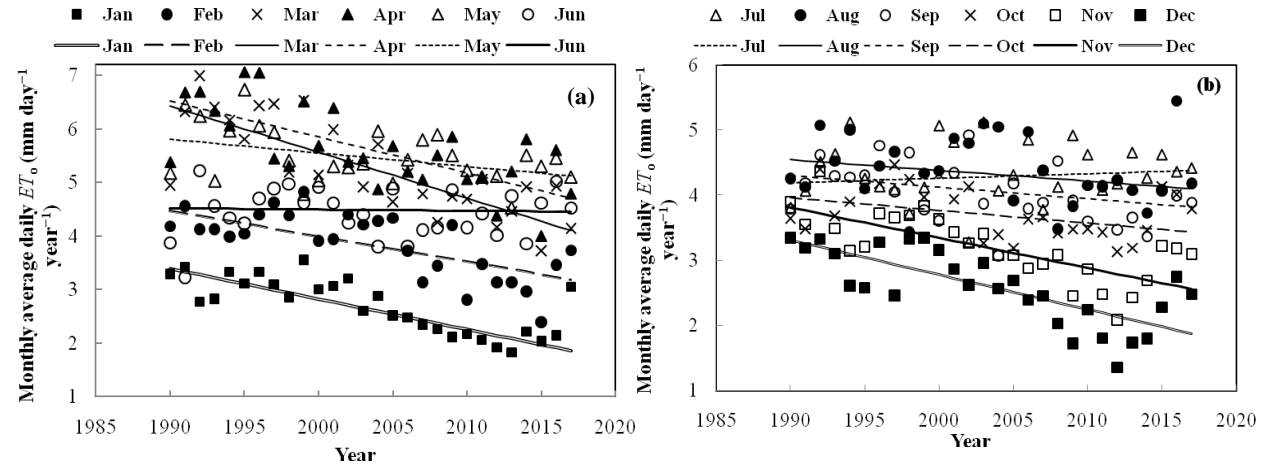
Fig. 2. Monthly average daily reference crop evapotranspiration, ET_o ( \text{mm day}^{-1} \text{ year}^{-1} ), over the study period (1990–2017) for the months of: (a) January to June and (b) July to December.
