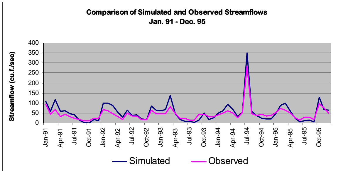
Figure 2 Observed Vs. simulated daily average streamflow, January 1991 - December 1995
