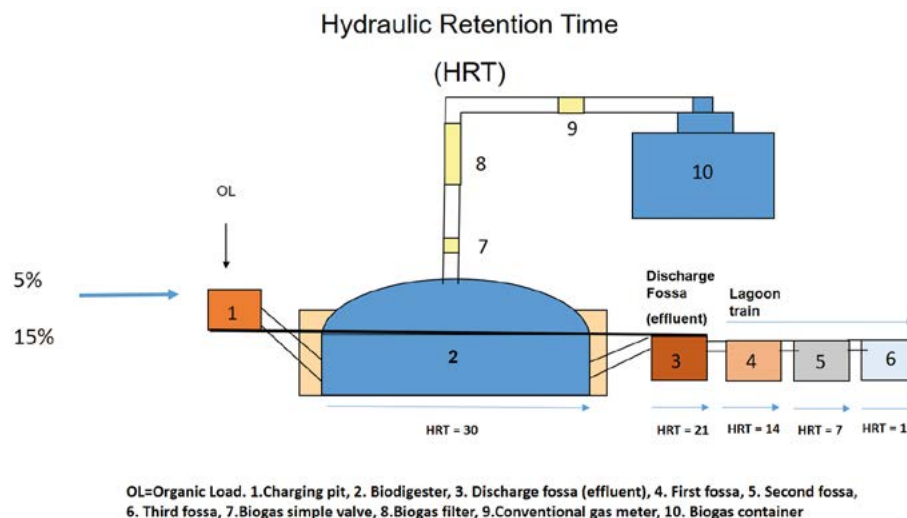
Figure 1. Schematic of the biodigester with three adjacent stabilization ponds (Image modified from Domínguez-Araujo et al. , 2023).
