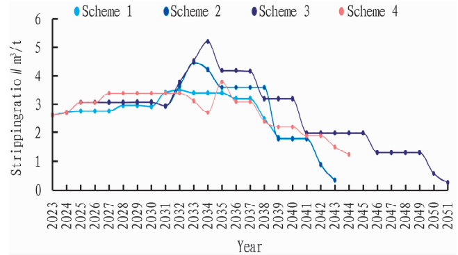
Fig. 10 Comparison of the stripping ratio of each scheme during the production period
