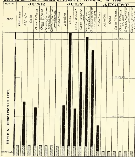
DIAGRAM SHOWING THE TIME OF IRRIGATION AND DEPTH OF WATER USED ON DIFFERENT CROPS AT LARAMIE, WYOMING, IN 1896.
