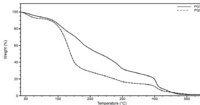
Figure 5. TGA curve of orange peel bioplastic films.
