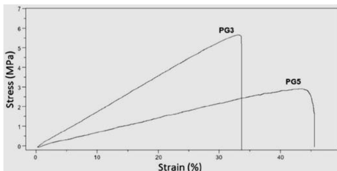
Figure 3. Stress-strain curve of bioplastic films.
