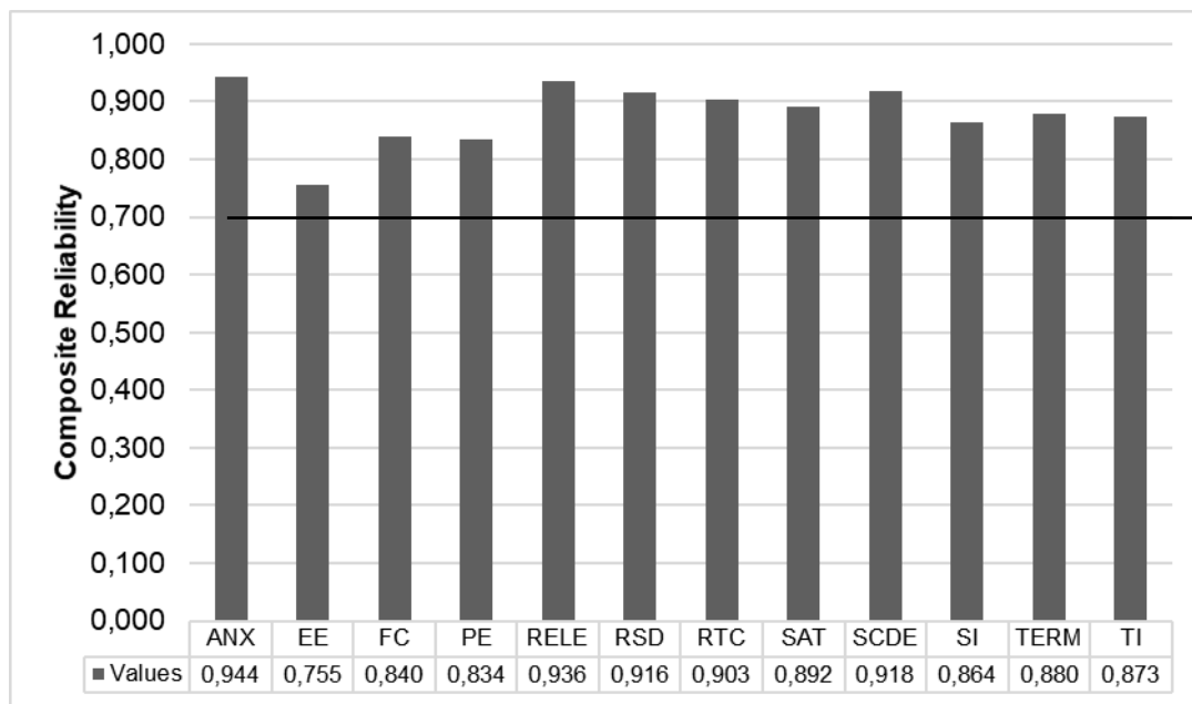
Figure 2. Composite Reliability
