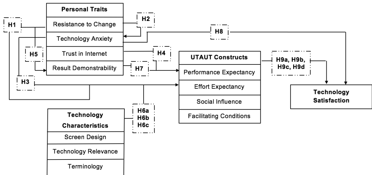
Figure 1. Research Model
