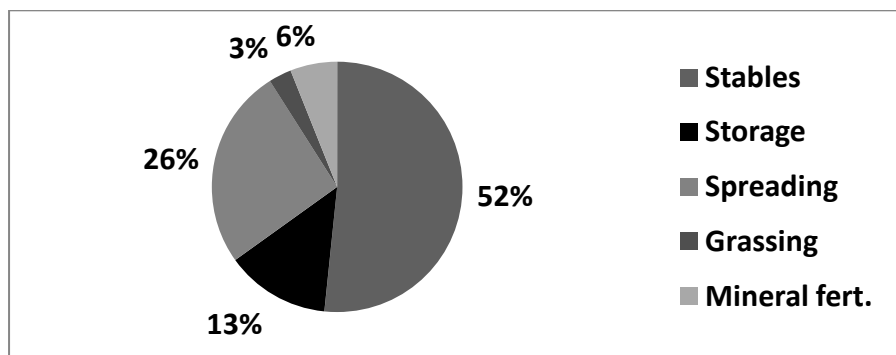
Figure 1. Ammonia emission from agriculture \text{NH}_3\text{-N} /year average 2003-2007 from different sources (plants are excluded)
