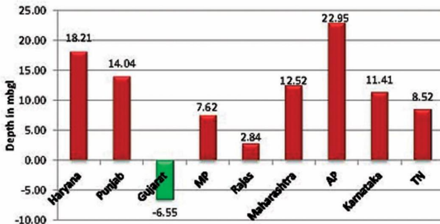
Figure 3. Change in Depth to Water Level between TE 2008-2009 and TE 2017-2018.
