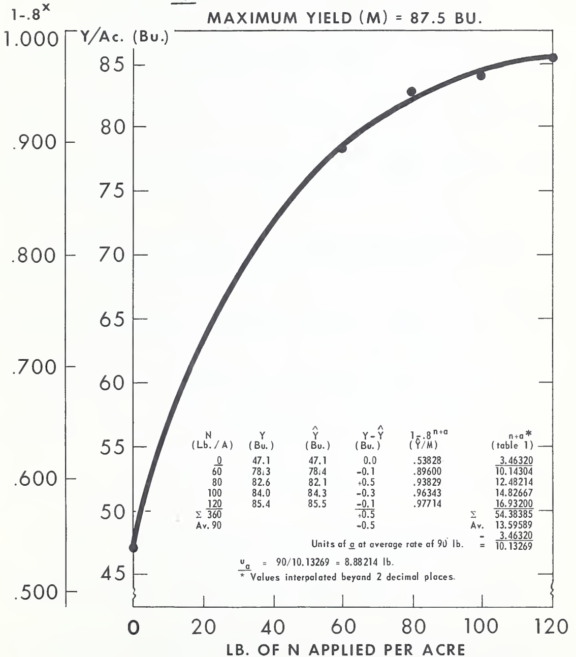
Fig.1 - Fit of a Standard Yield Curve to Corn Yield Response to Nitrogen and Calculation of Size of Unit, u_a Associated With R = 0.8
