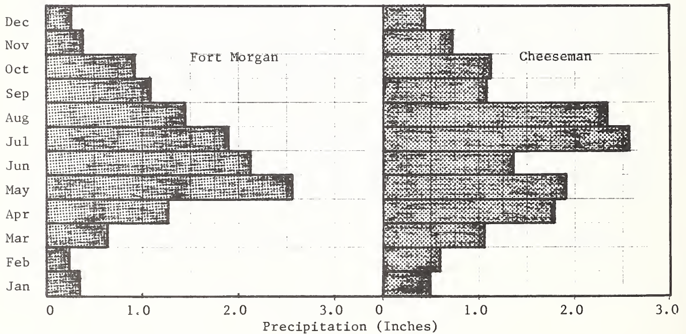
Figure A-1 Monthly Precipitation for Selected Locations
