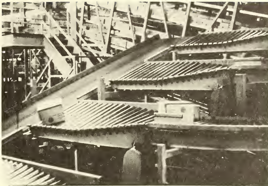
Figure 28.—Conveyors from selection level merging into one conveyor.
