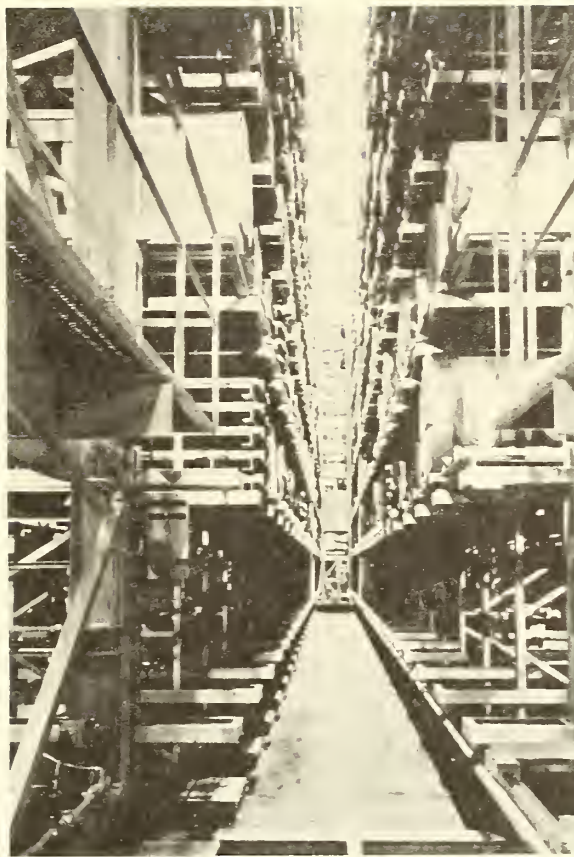
Figure 19.—Aisle and guide rail used for storage-retrieval machines.
