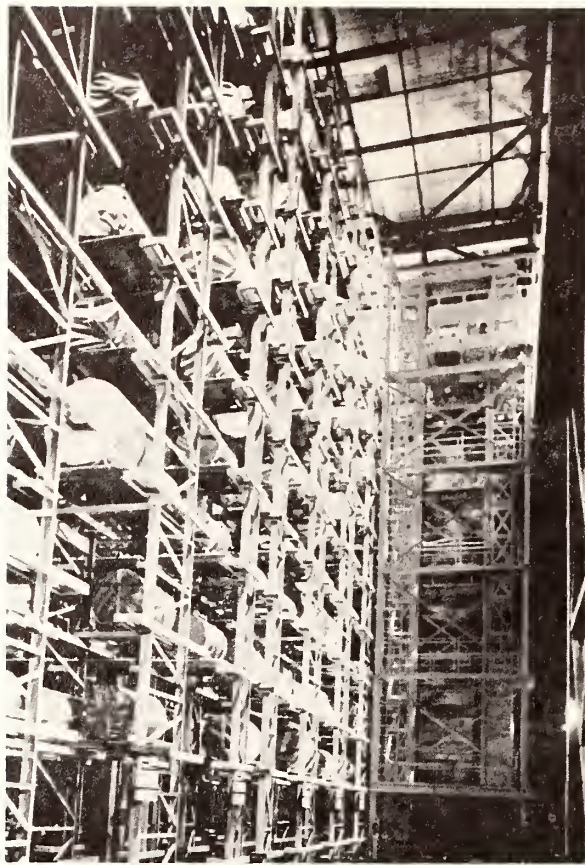
Figure 18.—Storage cells used with storage-retrieval machines.
