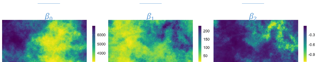
Figure 3. Spatial distribution of true yield response parameters (or “field characteristics”) in one simulation
