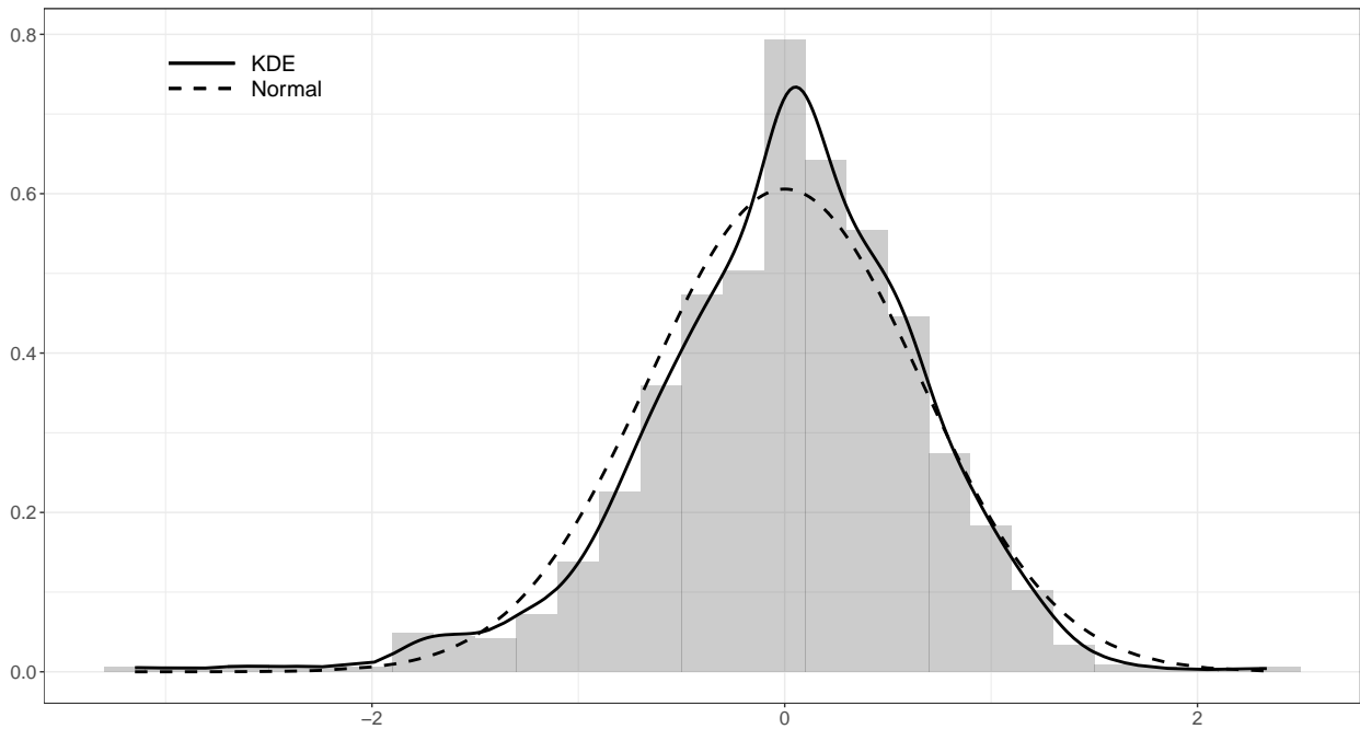
Figure 2: Equation (1): Residuals histogram; parametric (Normal) and non-parametric kernel density estimation (KDE)
