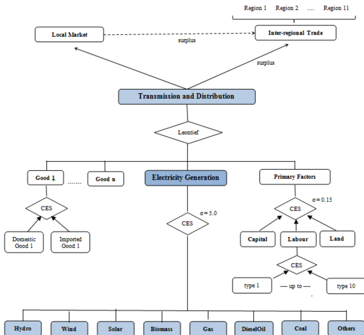
Figure 03 – Electricity production and trade mechanism in TERM-BR10.
