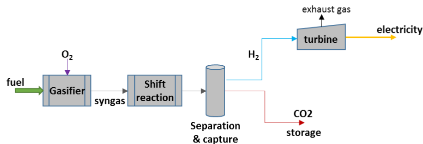
Figure 6. Pre-Combustion
