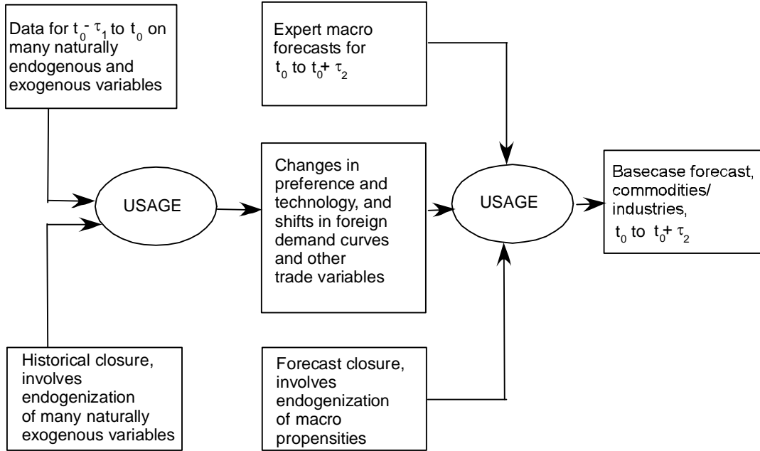
Figure 2.1 Relationship between Historical and Forecast Simulations
