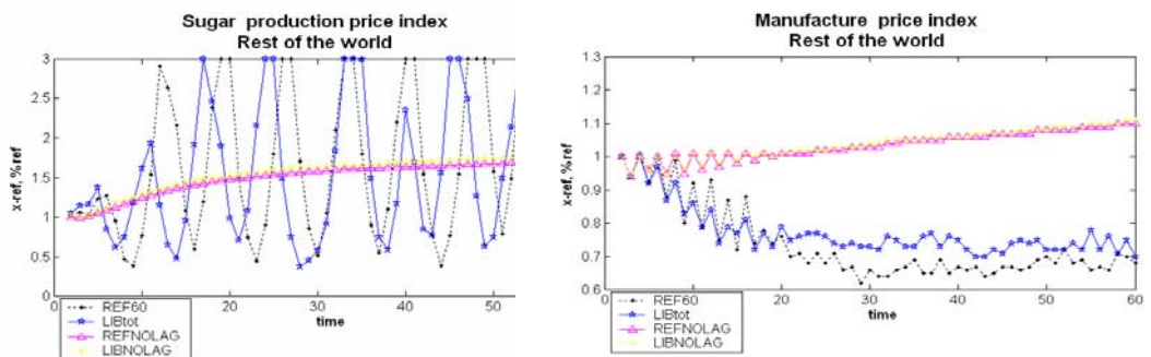
Figure 5 Prices of sugar and manufactures with four scenarios LIBNOLAG and LIBTot are liberalisation with and without perfect information. REFnolag and REF60 are corresponding reference runs
