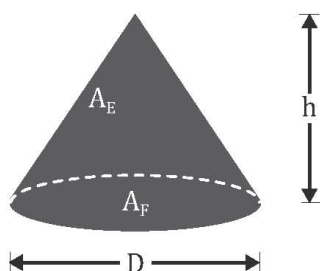
Figure 5-D-3: Equations for Calculating the Shape Factor for a Conical Manure Pile
