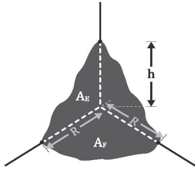
Figure 5-D-1: Equations for Calculating the Shape Factor for a 2-Sided Storage Bin with Quarter-Cone Pile
