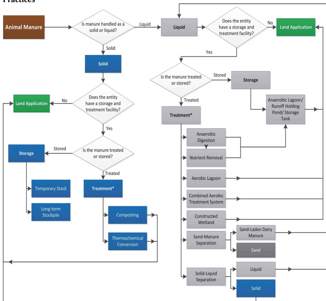
Figure 5-7: Schematic Structure of Possible Combination of Manure Storage and Treatment Practices
