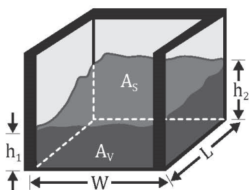
Figure 5-D-2: Equations for Calculating the Shape Factor for a 3-Sided Storage Bin
