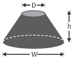
Figure 5-D-4: Equations for Calculating the Shape Factor for a Free-Standing, Truncated Conical Stack
