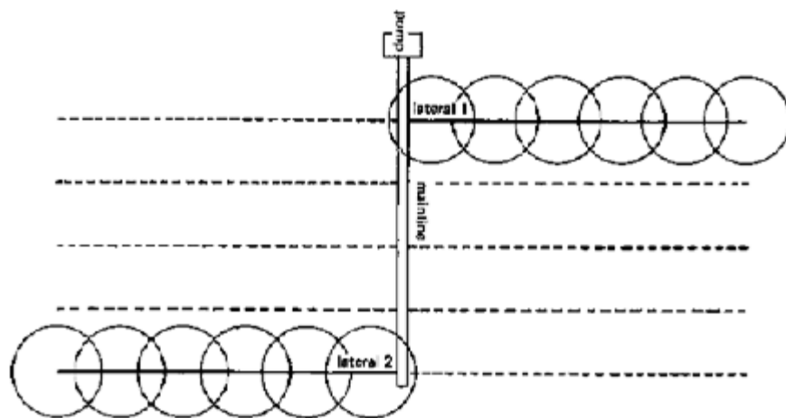
Figure 7.4: Example of layout for gun-spray sprinkler (Source: FAO, 1985)
