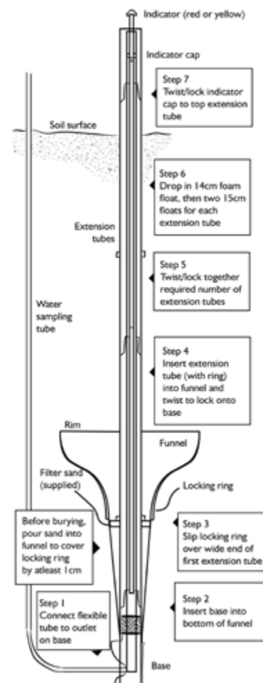
Figure 9.3. Installation steps
