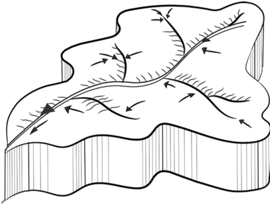
Figure 4.3: Sketch of catchment runoff generation model
