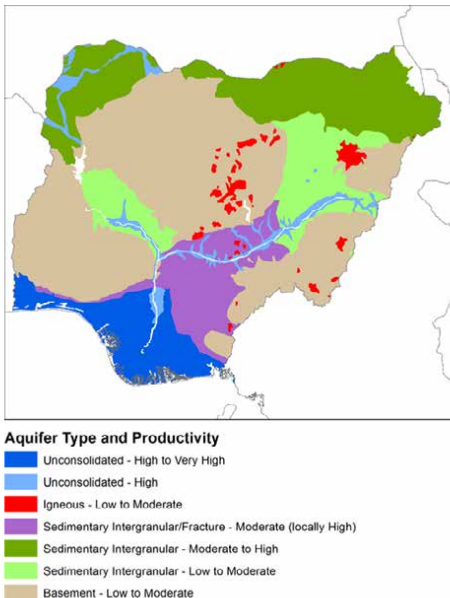
Figure 3.4: Example of a hydrogeological map showing aquifer productivity in Nigeria
