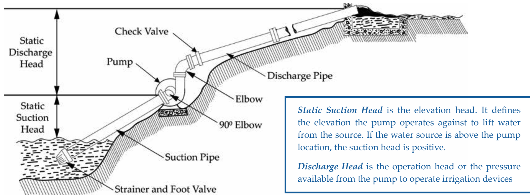
Figure 2.3: Basic layout of a typical surface water pumping (FAO, 1986)
