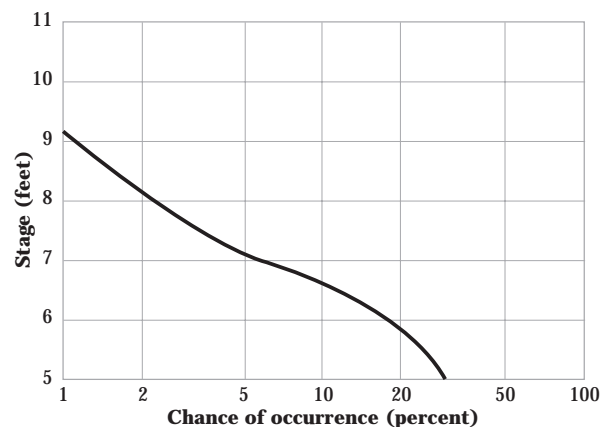
Figure 2-4 Stage–frequency curve
