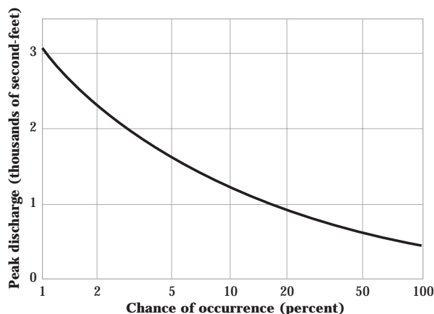
Figure 2-2 Discharge–frequency curve
