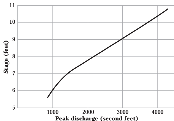
Figure 2-3 Discharge–stage curve
