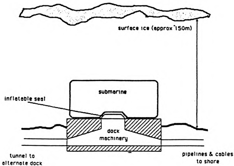
Figure 3 Submarine Docking Arrangement
