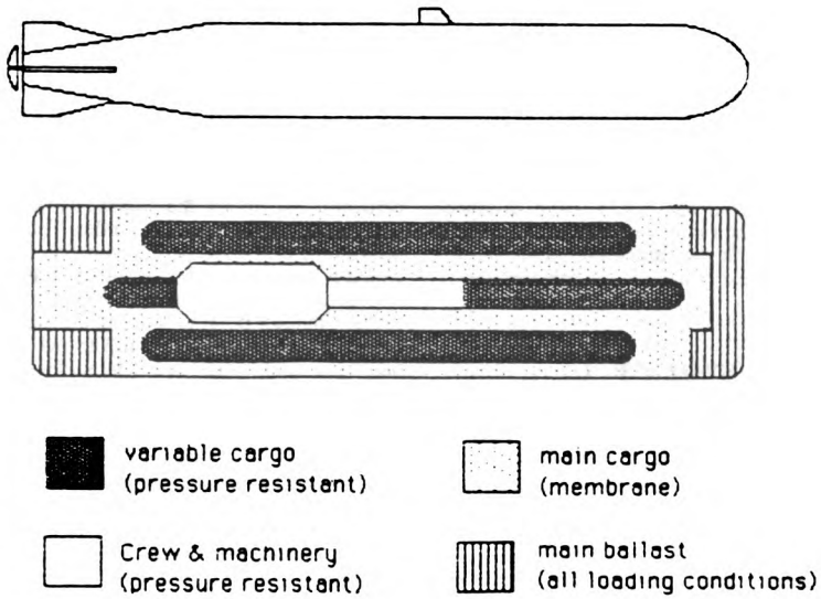
Figure 2 General Arrangement—Membrane Construction
