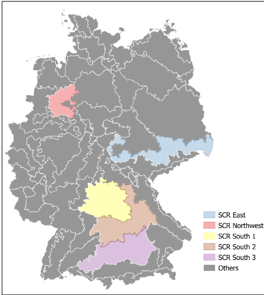
Figure 3: Soil-climate-regions (SCR) in Germany (ROBBERT et al., 2007) and presentation of the SCRs considered in this study
