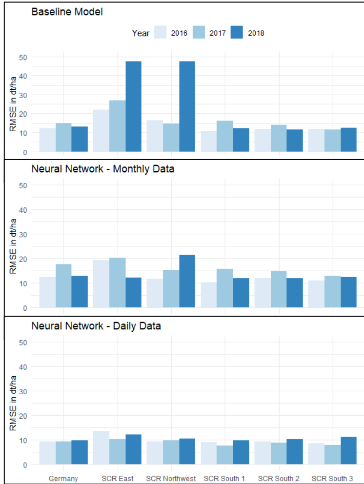
Figure 5: RMSE by year of the testing set for one model for all farms (Germany) and SCR-specific models
